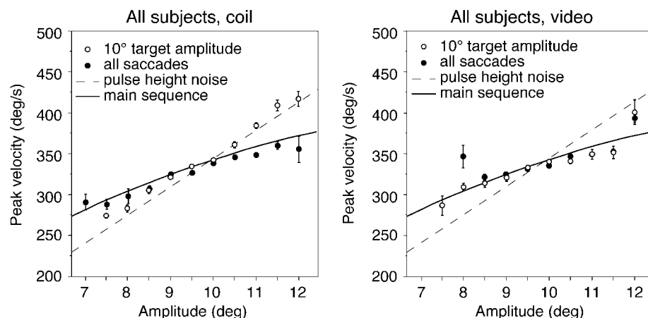
FIG. 4. Average behavior of our subjects measured with scleral coils (left) and video system (right). Peak velocities averaged for 0.5° wide bins of amplitude as a function of amplitude. ●, the peak velocity of all saccades as a function of target amplitude. Both systems reproduce the main sequence for our range of amplitudes very well. ○, the peak velocity of the saccades for which the target amplitude was between 9.5 and 10.5° as a function of saccade amplitude. — and — —, main sequence and pulse-height noise behavior predicted (see Table 1).
