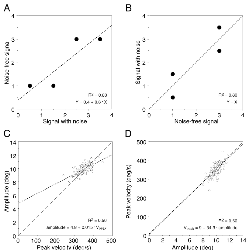
FIG. 2. The choice of the independent parameter influences the outcome of a regression analysis. A and B: regression to 4 data points with the variability either in the independent (A) or dependent (B) variable. The correlation coefficients are the same, but the slopes and intercepts differ considerably because a linear regression minimizes the vertical distance between the line and the data points. The regression theory assumes a situation as in B in which all variability is in the dependent variable. Note that the sum of the squared residuals (vertical distances) is smaller with the erroneous choice of independent variable (A). C and D: application to main sequence analysis. Two hundred model data points (the same set of points is used in both graphs) were generated according to the pulse-height noise model, with an average amplitude of 10^\circ and velocity 350^\circ/\text{s} . We assume that the pulse-height noise leads to a distribution of the saccades exactly along the dashed line with a SD of 6% in amplitude and velocity. We subsequently added normally distributed independent noise with SDs of 0.14^\circ to the amplitude and 25^\circ/\text{s} to the velocity values. We fitted a linear regression ( \cdots ) line through the data using either variable as independent variable. The regression with peak velocity as independent variable (C) suggests that pulse-height noise is not the main source of variability. However, if we use amplitude as the independent parameter (B), the linear regression recovers the pulse-height noise model that underlies the data.
