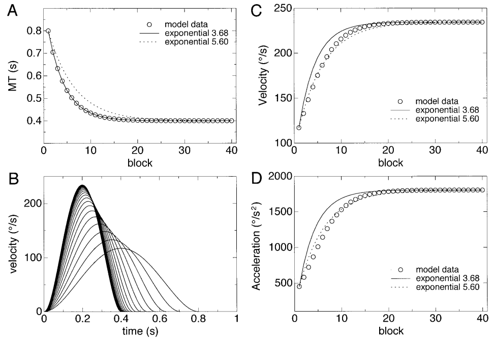
Fig. 1A–D A model for learning to move twice as fast as normal. The movement times reduce exponentially from 0.8 s to 0.4 s, with a time constant of 3.68 blocks. A The development of the movement time (circles). The continuous lines show exponential functions (two different time constants), with the same initial and final values as the model data. B Velocity profiles of 40 model movements. Each movement is representative of a learning block. C The development of the peak velocity. D The development of peak acceleration
